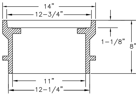
CAST IRON RING AND COVER
